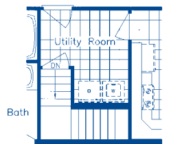
OPTIONAL BASEMENT/UTILITY ROOM WITH GABLE ENTRY
