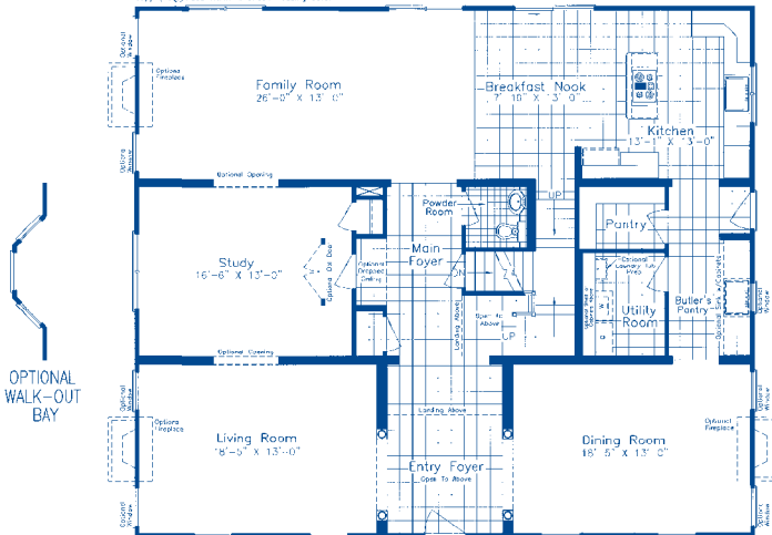
STANDARD BASEMENT PLAN
