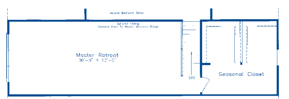
OPTIONAL 3rd FLOOR 9/12 ROOF AND STAIRS TO MASTER RETREAT
