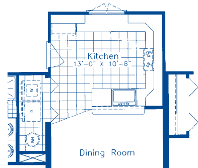
OPTIONAL KITCHEN LAYOUT
