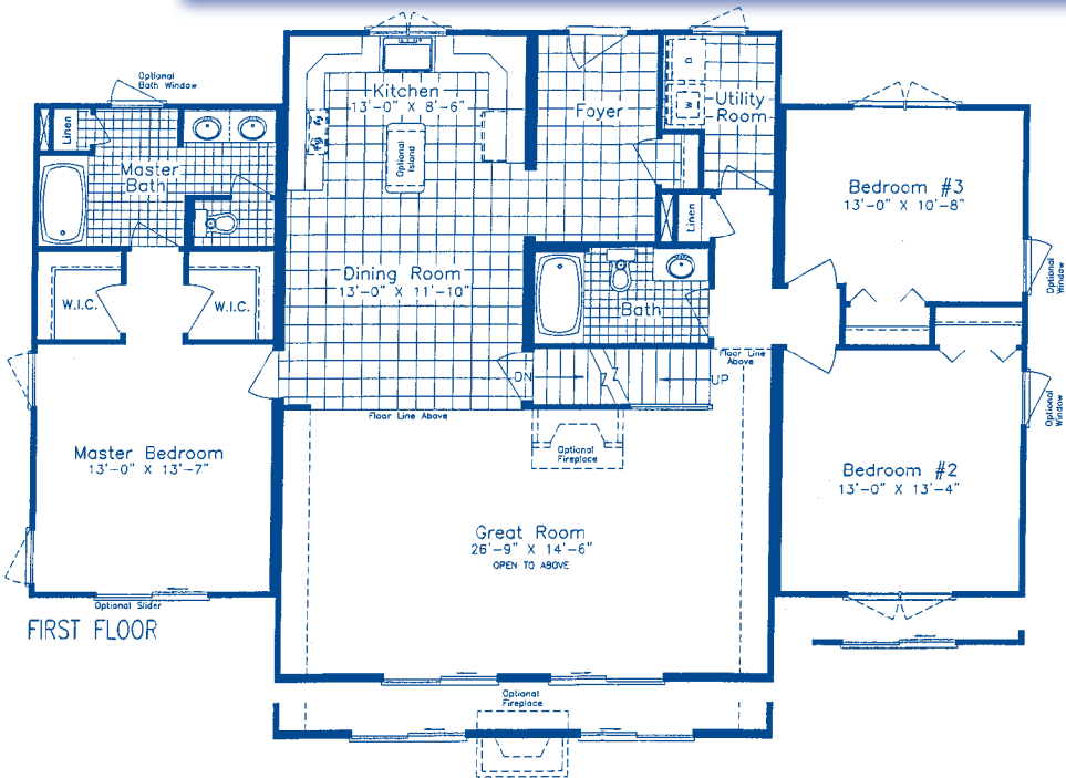
FIRST FLOOR OPTIONAL FIREPLACE LOCATION
